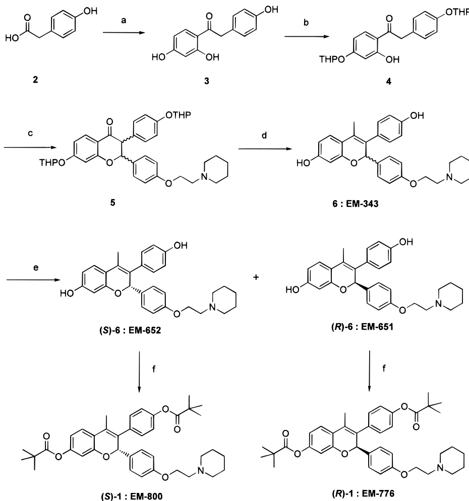
(S)-1 EM-800
